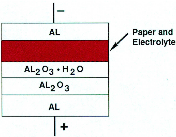
Fig. 1: As an aluminum electrolytic ages on the shelf, the aluminum-oxide dielectric material dissolves into the electrolyte causing leakage and dielectric absorption.
