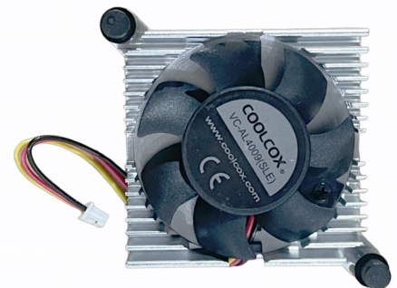
REPLACEMENT FAN 40MM X 40MM X 10MM 5200RPM HYDRAULIC BEARING 12-VOLT 5.8CFM 3-WIRE W/MOLEX CONN.
