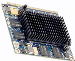
PCBA: GRAPHICS CARD, ATI MXM-1 M24-C 128MB, WMS BB2
